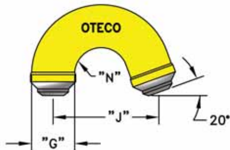
160° Standpipe Gooseneck (GSNK160)
