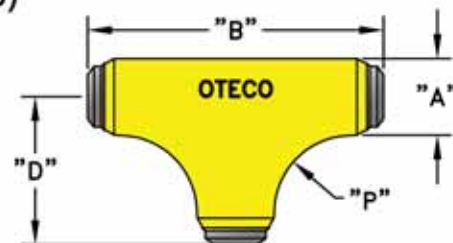
Long Sweep Full Flow Tee (LSFFT)
