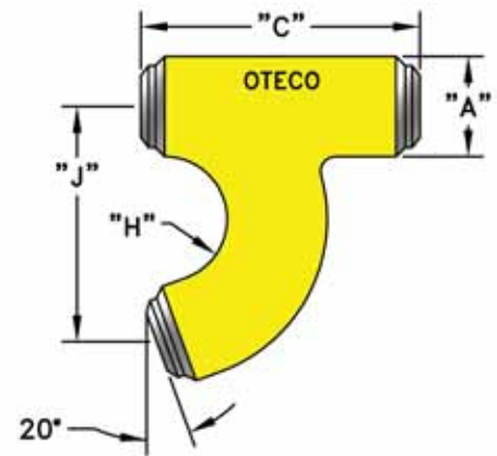
160° Standpipe Gooseneck with Top Outlet (GSNKTO)
